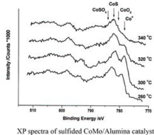
XP spectra of sulfided CoMo/Alumina catalyst
