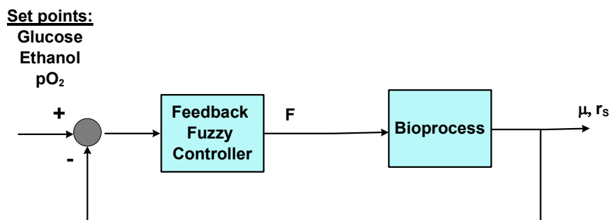
Fig.5 – Schematic presentation of the fuzzy control structure: F = real glucose feed rate [L/h], \mu = specific growth rate [ h^{-1} ], r_s = specific glucose consumption rate [g/L/s], Y_{X/S} = Y_{X/S} is the substrate conversion yield referred to the biomass [g cells as dry matter/ g substrate], pO_2 = dissolved oxygen concentration [mg/L].
