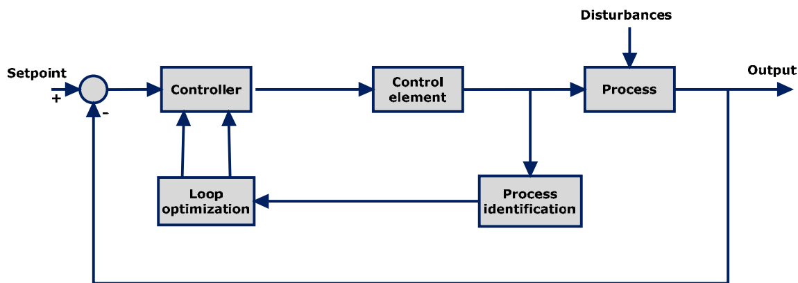
Fig.3 – Adaptive control structure.
