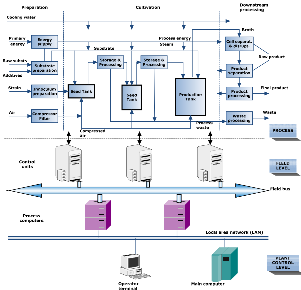
Fig. 1 – General presentation of the computerized bioprocess control 2 .
