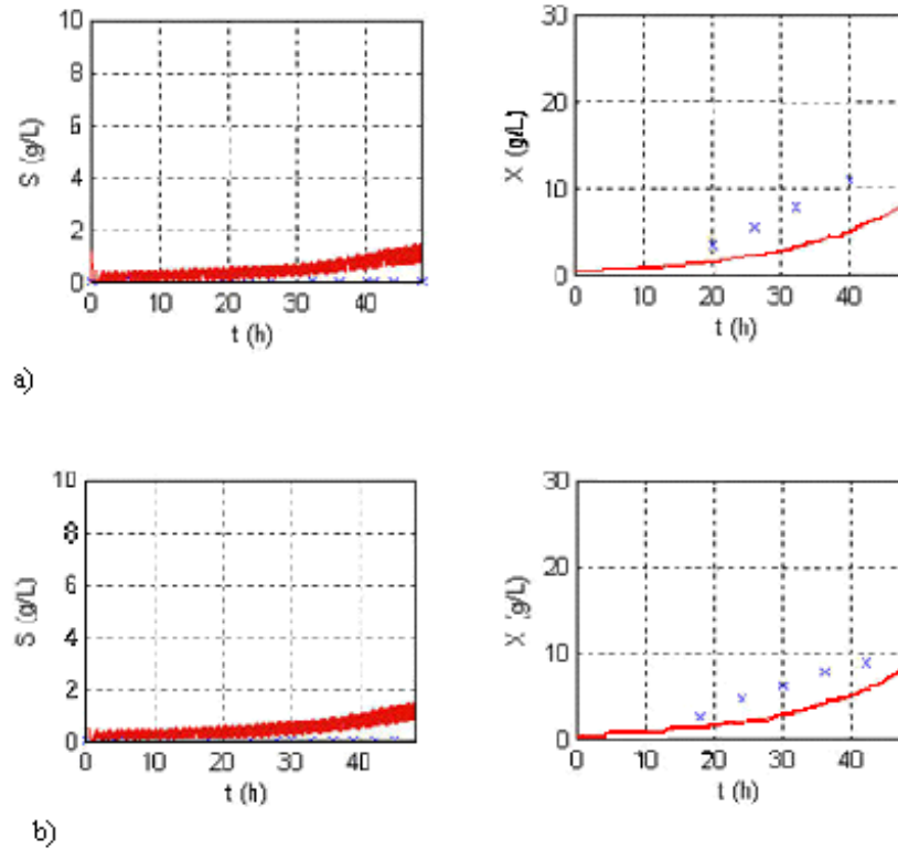
Fig. 6 – Simulation results of the control loop: a) first experiment; b) second experiment; ('-' – simulation results; 'x' – experimental data).
