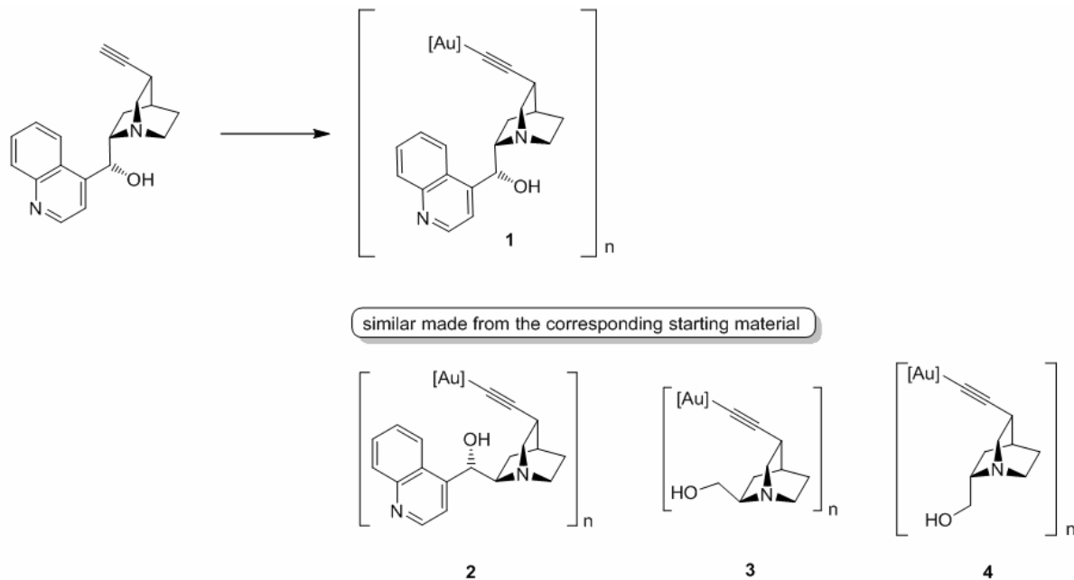
Scheme 2 – Synthesis of gold(I)-polymeric derivatives 1-4.
