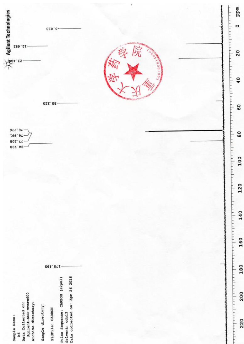
Fig. 1The ^{13}\text{C} NMR of C
