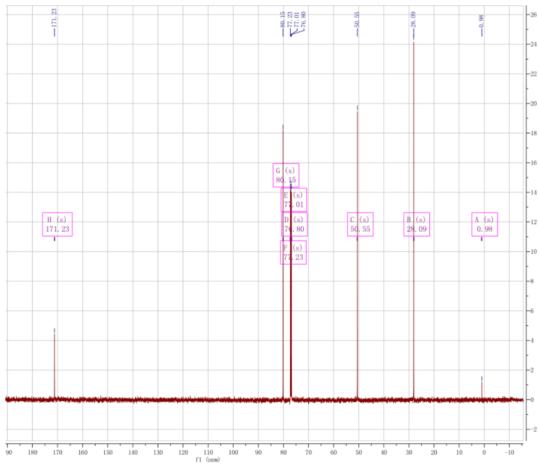
Fig.6 The ^{13}\text{C} NMR of D
