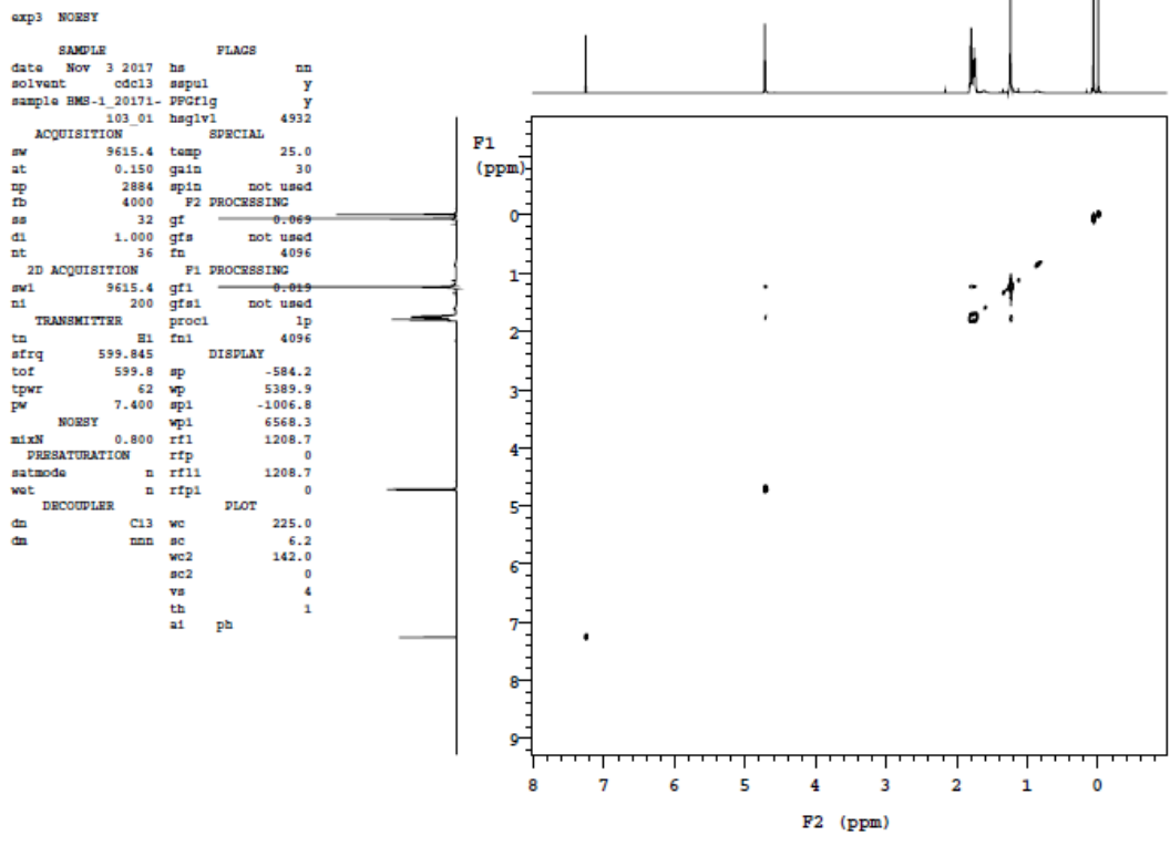
Fig.3 The NOESY of C
