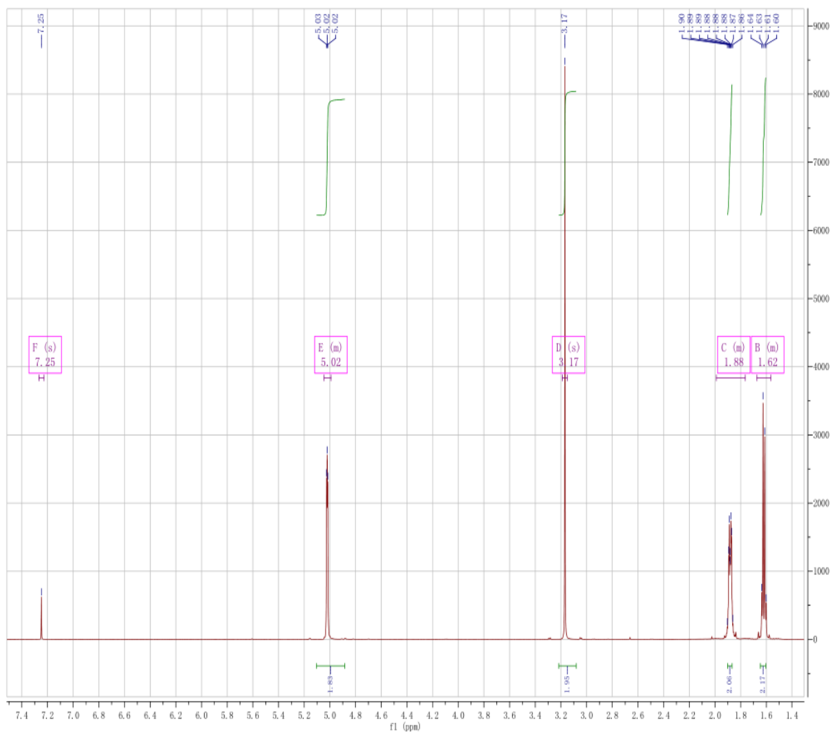
Fig.5 The 1 H NMR of D
