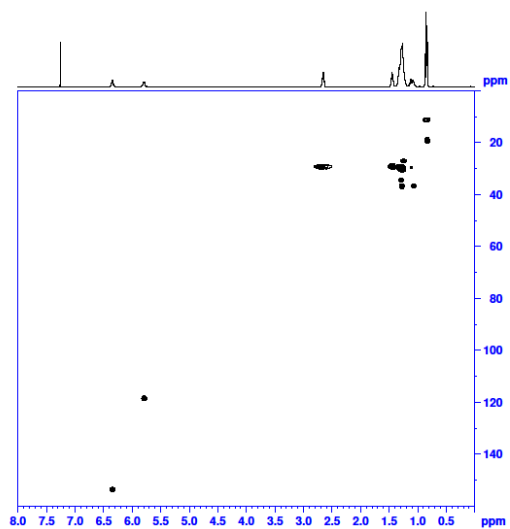
Figure3 ^1\text{H} NMR of FDSF
