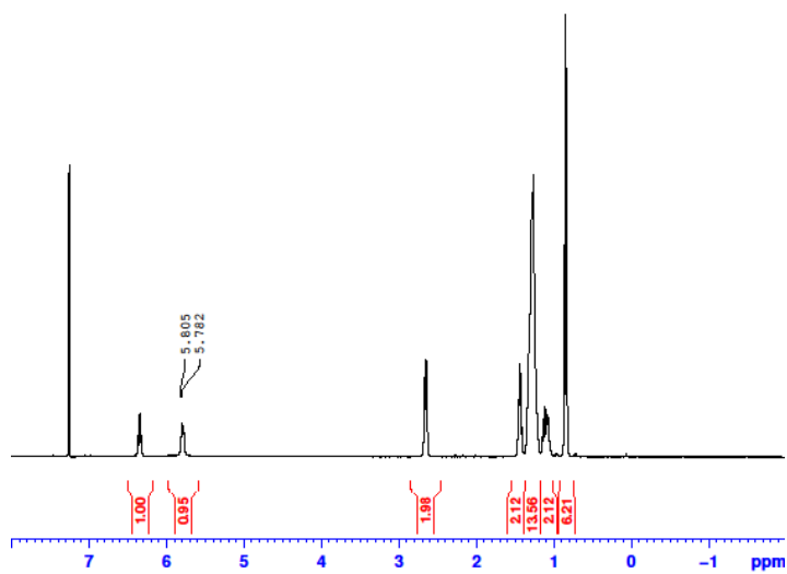
Figure2 ^{13}\text{C} NMR of FDSF
