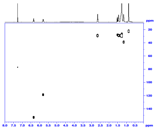
Figure 9 ^1\text{H} NMR of GDSF
