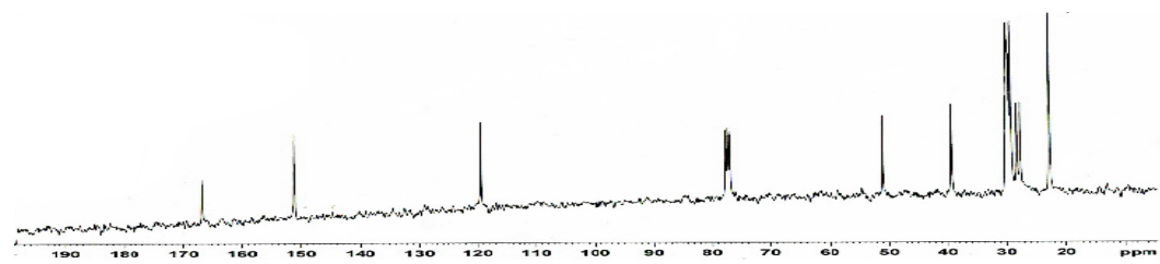
Figure 8 ^{13}\text{C} NMR of GDSF
