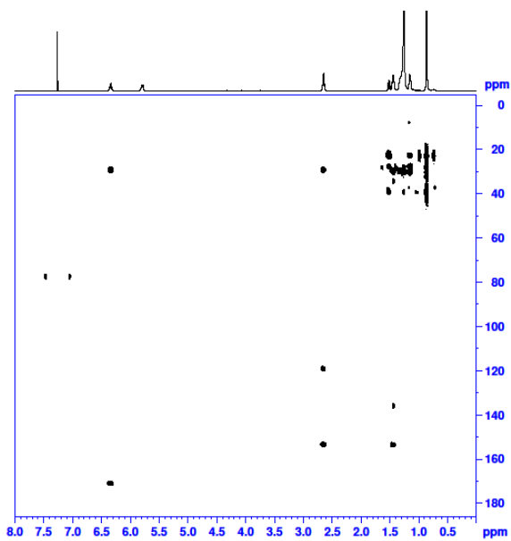
Figure 9 ^1\text{H} NMR of GDSF
