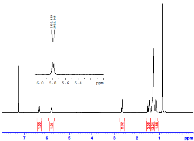
Figure 8 ^{13}\text{C} NMR of GDSF
