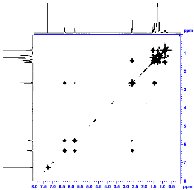
Figure 11 HMBC of GDSF
