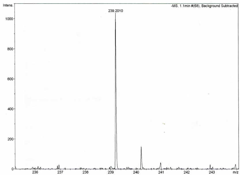
Figure 7 HRMS of GDSF
