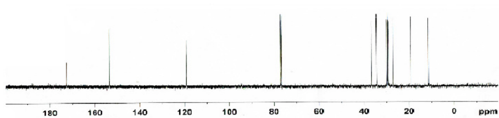
Figure2 ^{13}\text{C} NMR of FDSF
