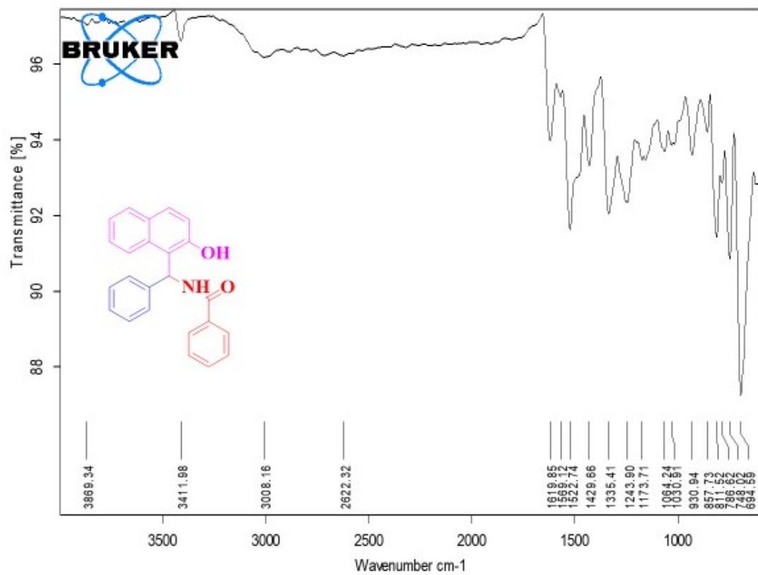
IR Spectrum of compound 4b , Table 3
