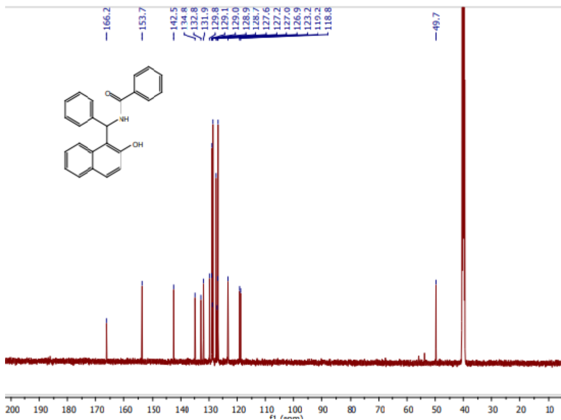
13 C NMR Spectrum of compound 4b, Table 3
