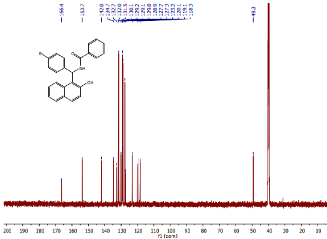
^{13}\text{C} NMR Spectrum of compound 4i , Table 3
