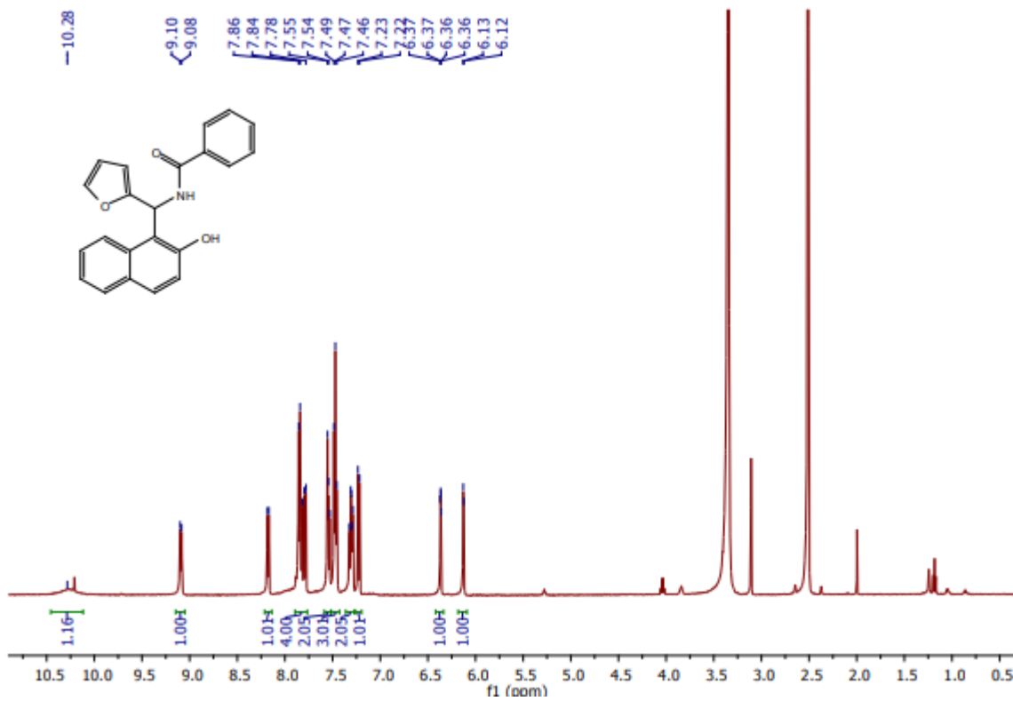
1 H NMR Spectrum of compound 4k, Table 3
