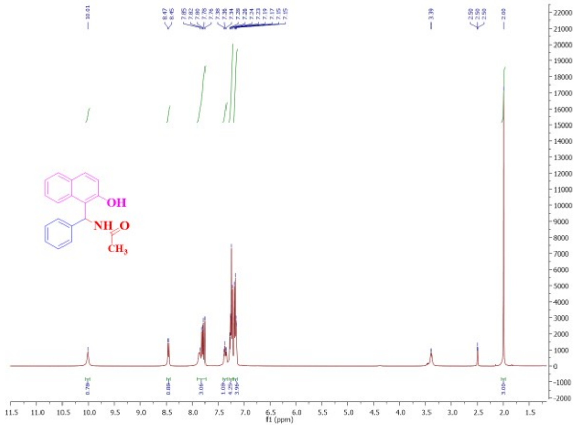
1 H NMR Spectrum of compound 4a, Table 3
