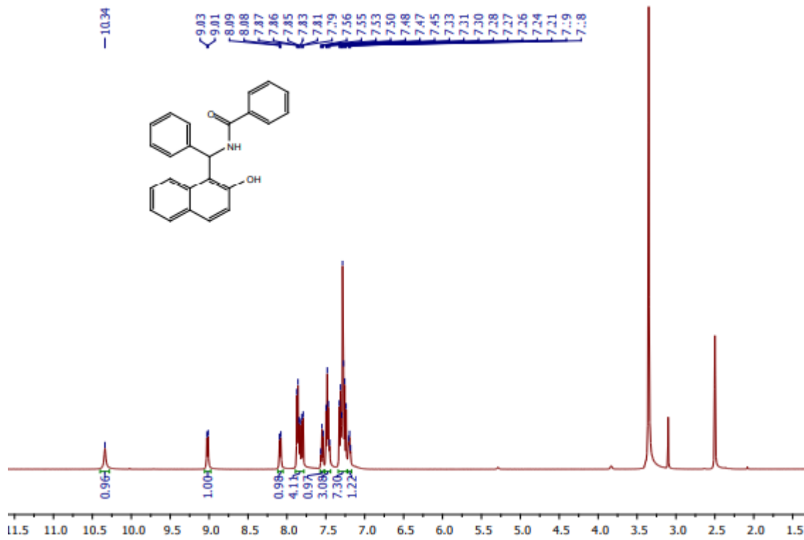
1 H NMR Spectrum of compound 4b , Table 3
