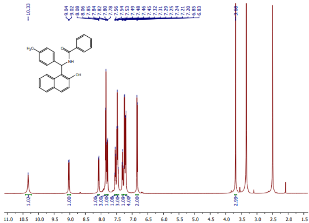
1 H NMR Spectrum of compound 4e, Table 3
