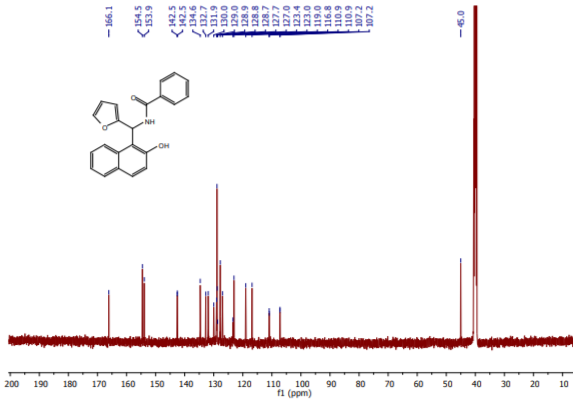
13 C NMR Spectrum of compound 4k, Table 3
