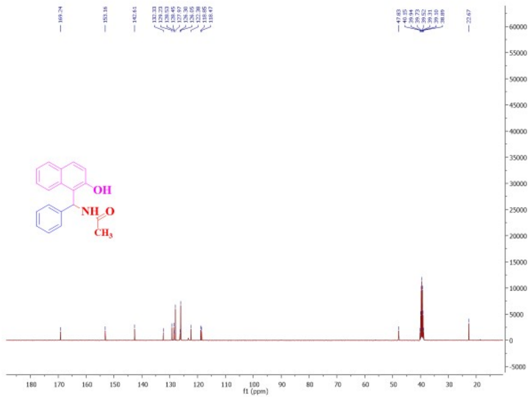
^{13}\text{C} NMR Spectrum of compound 4a, Table 3
