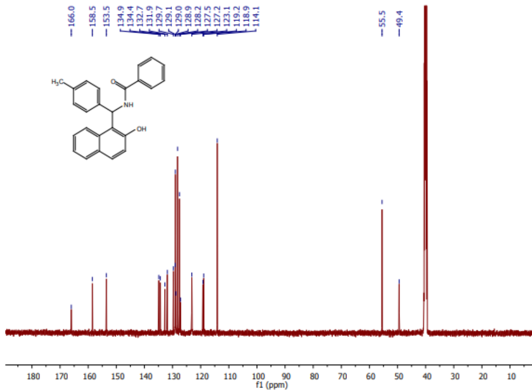
13 C NMR Spectrum of compound 4e, Table 3
