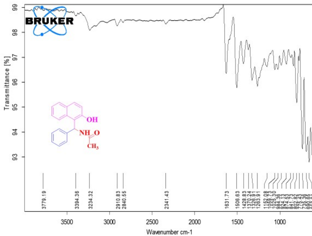
IR Spectrum of compound 4a , Table 3
