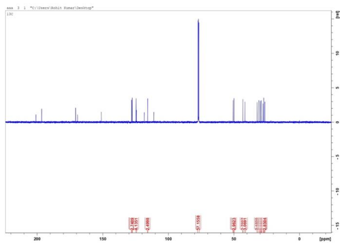
13 C NMR spectrum of compound 3a
