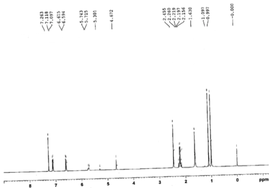
^1\text{H} NMR spectrum of compound 5d
