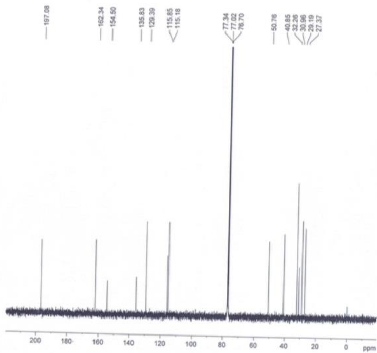
^{13}\text{C} NMR spectrum of compound 5d
