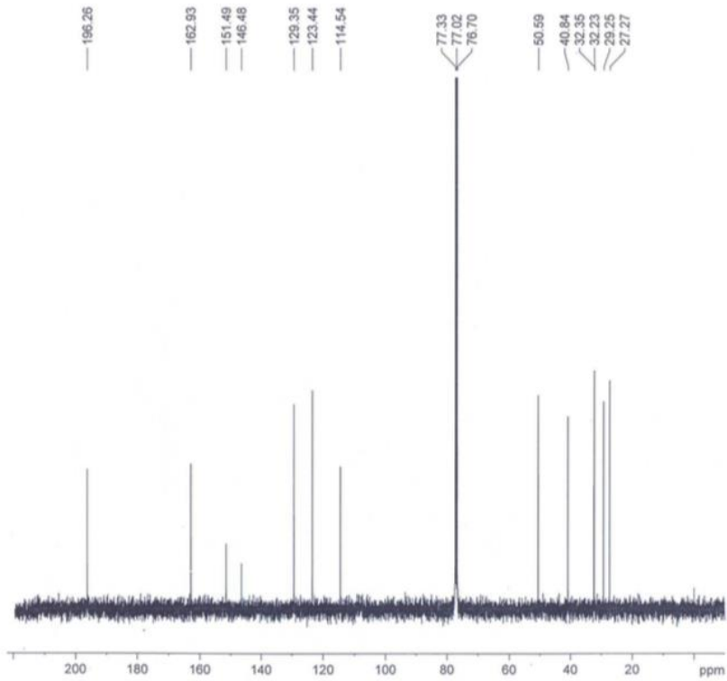
^1\text{H} NMR spectrum of compound 5e
