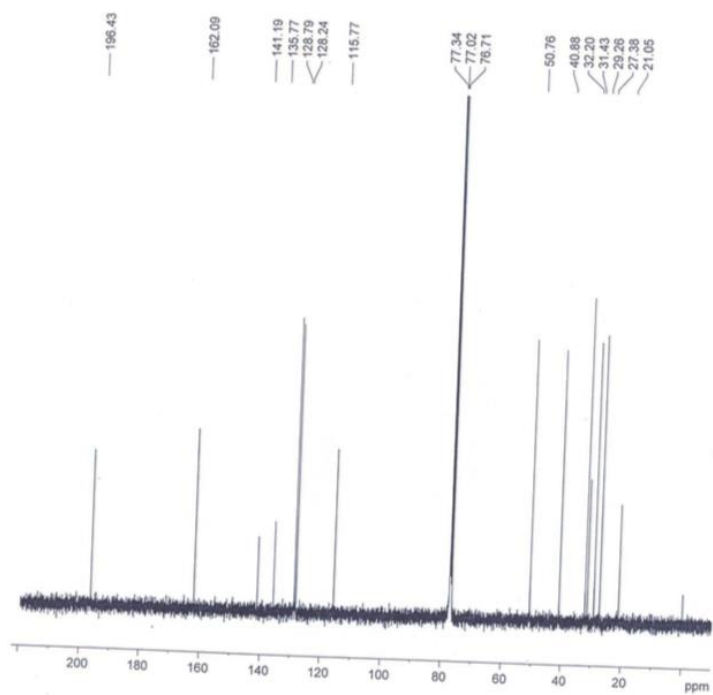
^{13}\text{C} NMR spectrum of compound 5h
