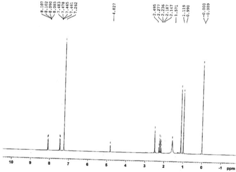
^1\text{H} NMR spectrum of compound 5e
