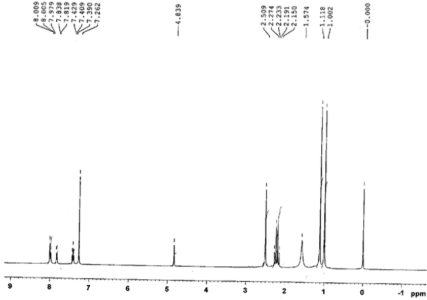
1 H NMR spectrum of compound 5b
