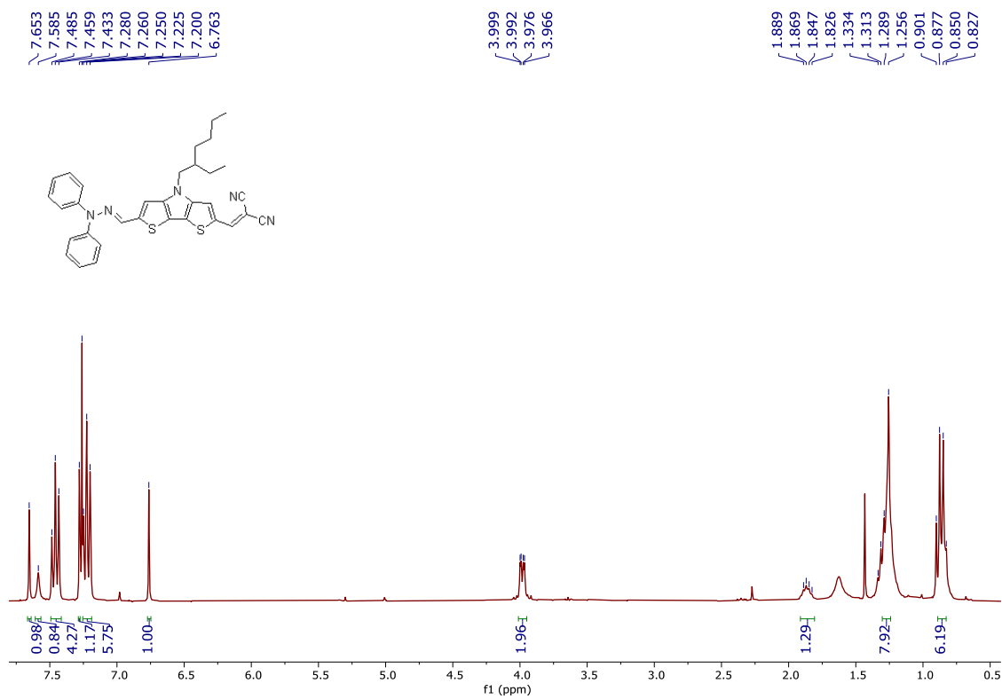
Figure S4a. 1 H NMR (CDCl 3 , 300 MHz) spectrum of 2
