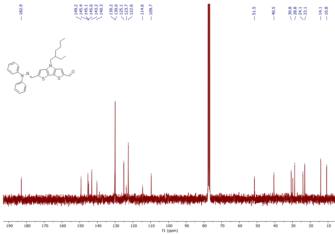
Figure S2b. 13 C NMR (CDCl 3 , 75 MHz) spectrum of 5b
