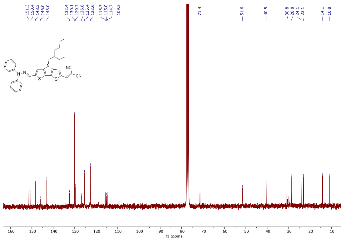
Figure S4b. 13 C NMR (CDCl 3 , 75 MHz) spectrum of 2
