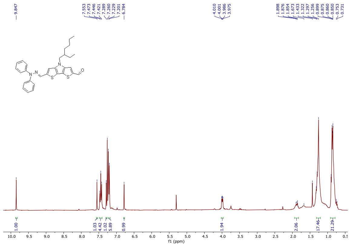
Figure S2a. 1 H NMR (CDCl 3 , 300 MHz) spectrum of 5b
