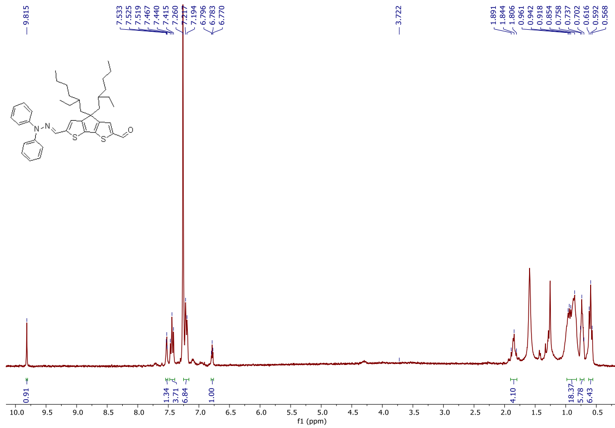
Figure S1a. 1 H NMR (CDCl 3 , 300 MHz) spectrum of 5a
