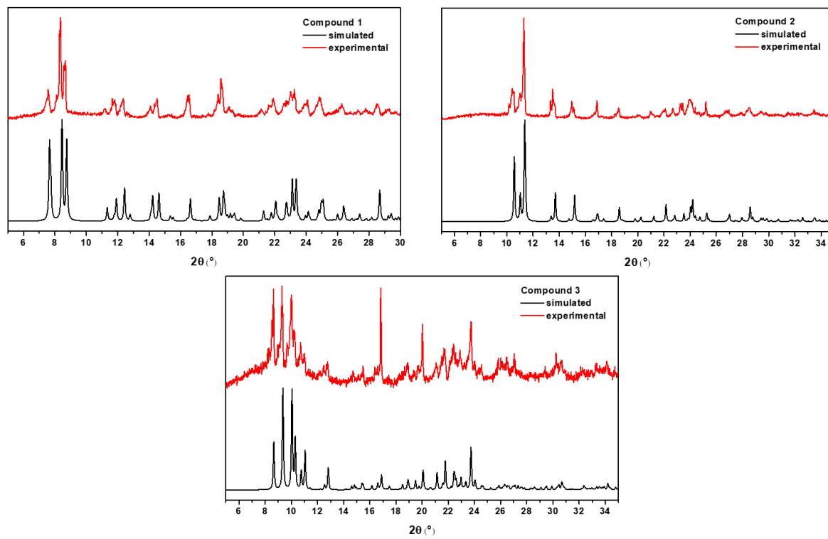
Fig. S1. Powder X-Ray diffractograms for compounds 1 – 3.
